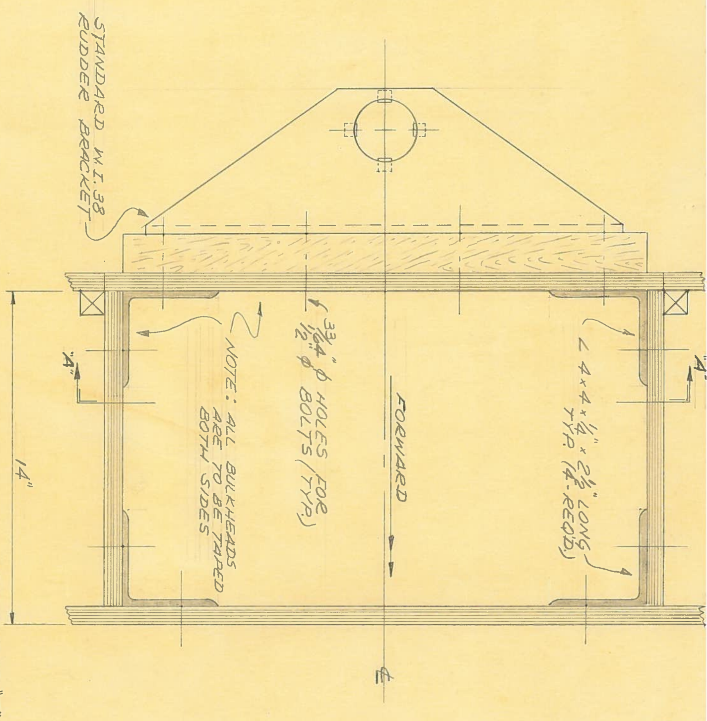
SECTION "A"-A"
